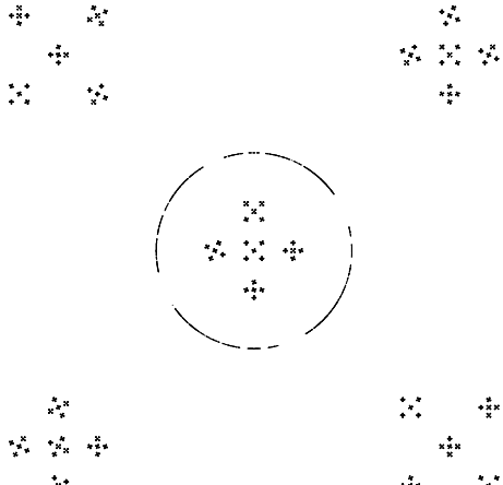
FIG. 2. A fractal of dimension 1 in 2-space, and its projection onto a circle. There are 7 levels of recursion.
