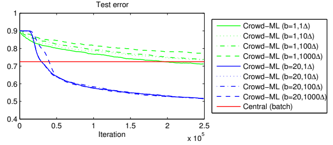
Fig. 9: Impact of delays on Crowd-ML with privacy ( \epsilon^{-1} = 0.1 ), varying minibatch sizes, and varying delays.
