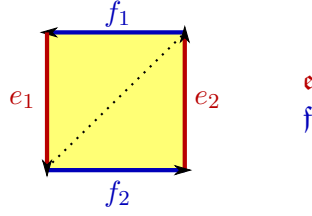
FIGURE 3. The symplectic double groupoid integrating the Lie-Poisson structures on E and F .
