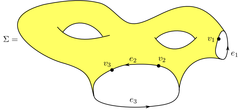
FIGURE 2. The marked surface (\Sigma, V) , with V = \{v_1, v_2, v_3\} . The boundary graph \Gamma has edges E_\Gamma = \{e_1, e_2, e_3\} and vertices V_\Gamma = V .
