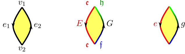
FIGURE 17. The Poisson homogeneous space corresponding to the Lagrangian Lie subalgebra \mathfrak{h} \subseteq \mathfrak{g} . The holonomies g \in G and e \in E satisfy eg = 1 .
