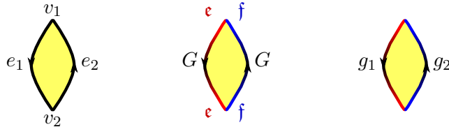
FIGURE 15. The double Poisson Lie group. The holonomies g_i \in G satisfy g_1 g_2 = 1 .
