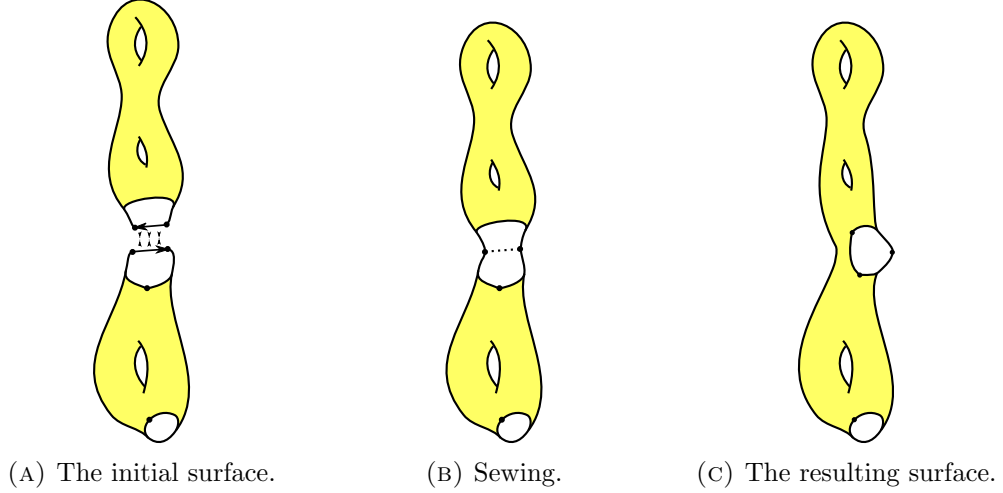
FIGURE 22. Sewing two edges from \Sigma . The two edges must have opposite orientation to ensure that the resulting surface is orientable.
