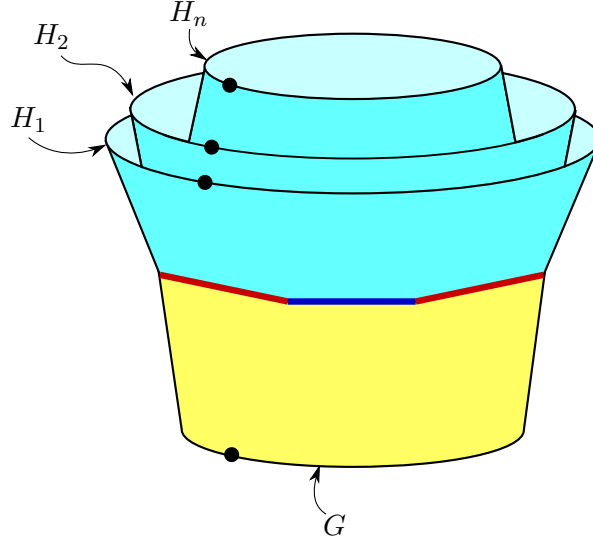
FIGURE 9. A branched surface which arises in the work of Philip Boalch (see [11, Pg. 2675] and [12, Fig. 2]).
