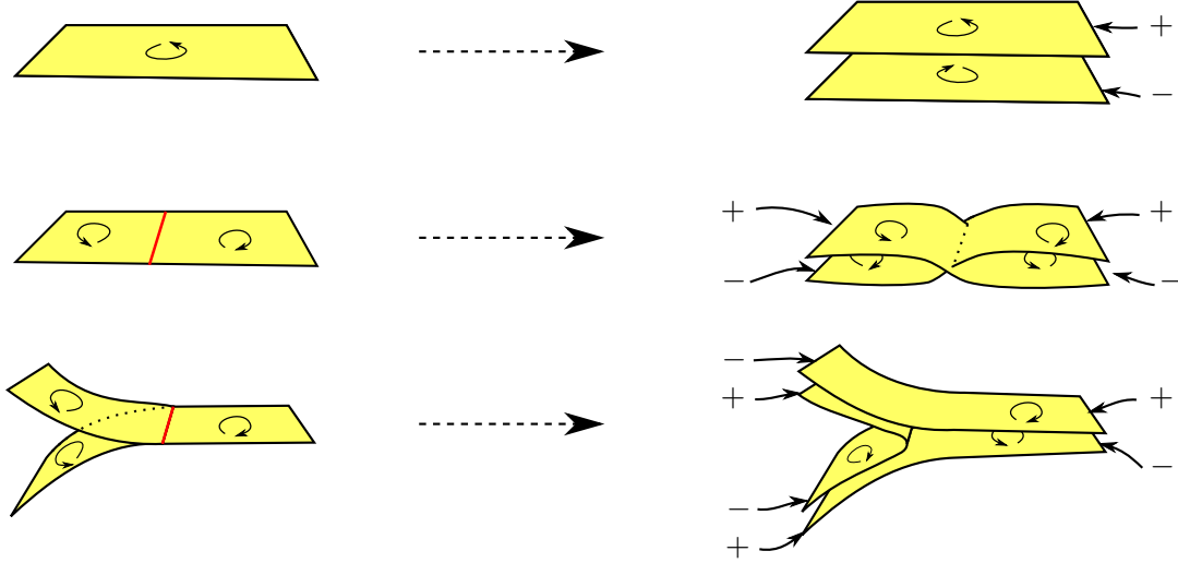
FIGURE 11. We replace each domain in our branched surface by two copies, one with the same orientation (labelled +), and one with the opposite orientation (labelled -). Each \mathfrak{c}_n -coloured domain wall is replaced by cyclically gluing the incident sheets together, respecting the orientations. In this way we obtain an oriented surface from our \mathfrak{c}_n -coloured (branched) surface.
