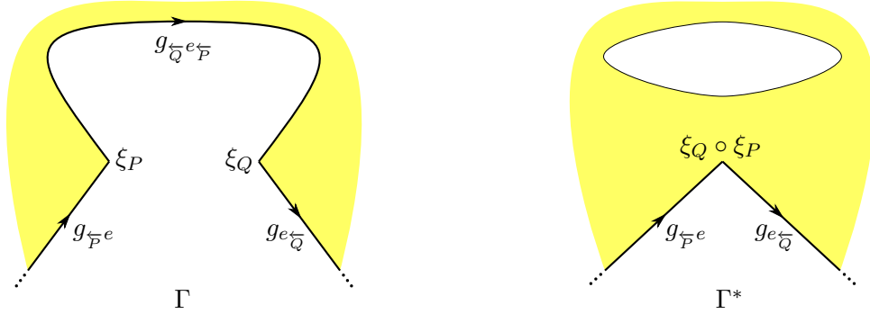
FIGURE 26. The graph \Gamma^* is the permutation graph obtained from \Gamma by deleting the edge, \overleftarrow{Q}e\overleftarrow{P} , passing from P to Q , and identifying the vertices P and Q . (The graphs are isomorphic outside the pictured regions.) Heuristically, we have obtained the graph \Gamma^* by gluing short sections from both ends of \overleftarrow{Q}e\overleftarrow{P} together (effectively divorcing it from the graph).
