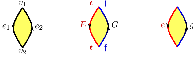
FIGURE 16. The Poisson Lie group. The holonomies g \in G and e \in E satisfy eg = 1 .
