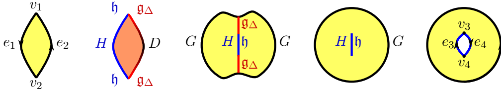
FIGURE 20. The dual Poisson Lie group, H . The holonomies h_1, d_2 \in D = G \times G along the edges e_1 and e_2 (respectively) satisfy h_1 d_2 = 1 , with h_1 \in H ; while the holonomies g_3, g_4 \in G along the edges e_3 and e_4 satisfy (g_3^{-1}, g_4) \in H
