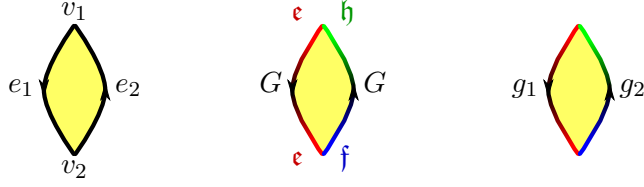
FIGURE 18. The affine Poisson structure on G . The holonomies g_i \in G satisfy g_1 g_2 = 1 .
