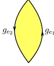
FIGURE 14. The cyclic product of holonomies, g_{e_2}g_{e_1} , is trivial, so g_{e_2} = g_{e_1}^{-1} .
