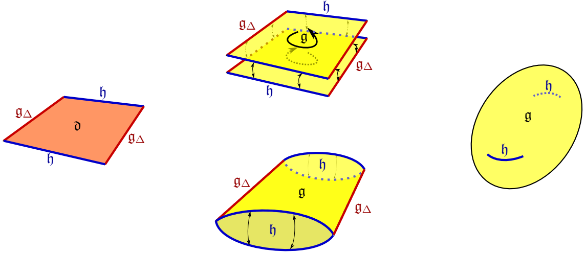
FIGURE 12. The moduli spaces for the quilted surfaces pictured above may each be identified with the Lu-Weinstein double symplectic groupoid integrating the Lie-Poisson structures on G and H . In the leftmost quilted surface, a single domain carries the structure Lie algebra \mathfrak{d} , while each of the domains in the other quilted surfaces carry the structure Lie algebra \mathfrak{g} . The double-ended arrows between edges in the middle two quilted surfaces signify that those pairs of edges have been coloured by the corresponding Lagrangian relations. The rightmost quilted surface depicts a sphere containing two domain walls each coloured by \mathfrak{h} .
