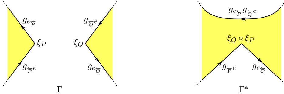
FIGURE 27. The graph \Gamma^* is the permutation graph obtained from \Gamma by identifying the vertices P and Q and composing the edge entering Q with the edge leaving P . (The graphs are isomorphic outside the pictured regions.) Heuristically, we have obtained the graph \Gamma^* by gluing a short section of the edges e\overleftarrow{P} and \overleftarrow{Q}e together.
