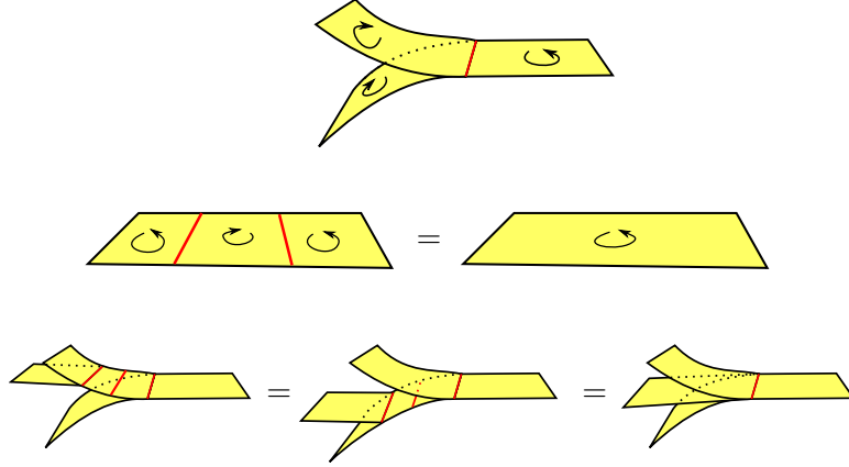
FIGURE 10. Each of the edges above are coloured by \mathfrak{c}_n , where n is the number of domains branching off the given edge. As we cross a branch locus, the orientation of the domains reverses. As depicted, we may move branch loci past each other.
