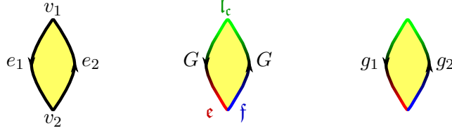
FIGURE 19. Lu-Yakimov Poisson homogeneous spaces. The holonomies g_i \in G satisfy g_1 g_2 = 1 .
