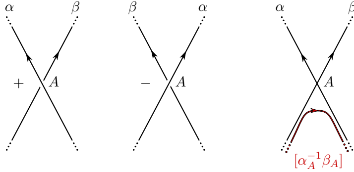
FIGURE 13. \text{sign}(A) = \pm 1 is determined by comparing the orientation of \alpha and \beta with that of \Sigma . The path [\alpha_A^{-1}\beta_A] is shown to the right.
