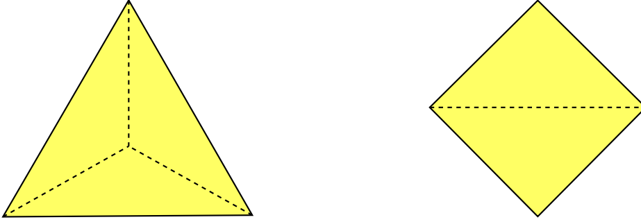
(A) A triangulation of the 3-gon.
