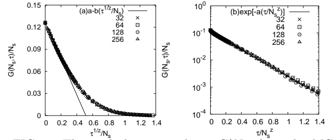
FIG. 9. The parked car correlator G(N_s, \tau) in the MC phase, for small \tau (a), it decays linearly as function of \tau^{1/z}/N_s , and for large \tau (b), it exponentially as function of \tau/N_s^z , where z = 3/2 . The data are obtained at \rho_o = 0.75 and \alpha = 1 .
