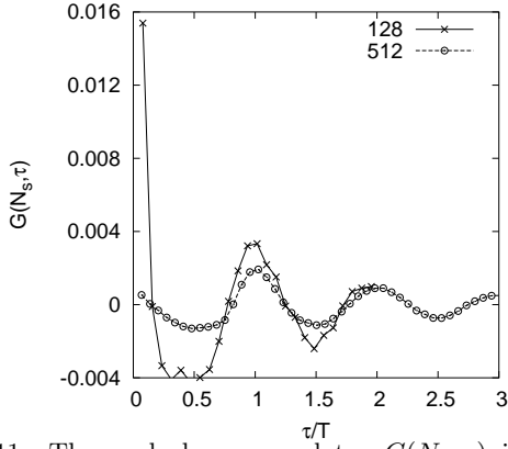
FIG. 11. The parked car correlator G(N_s, \tau) in the N phase; the garage is no longer macroscopically occupied, such that G does not scale with N_s any more. The correlations light up, like a lighthouse beam, at every time-of-flight interval \tau_{\text{flight}} = T . The data are obtained at \rho_o = 0.25 and \alpha = 1 .
