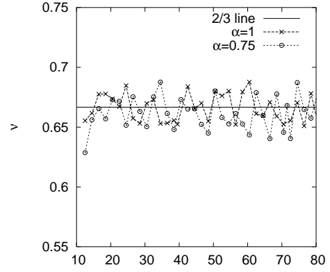
FIG. 8. Effective (finite-size-scaling type) value for the exponent \nu of the density profiles at the beginning of the road: \nu = 0.66(1) at \rho_o = 1/2 and \alpha = 1 (or 0.75 ). At the MC - N phase boundary, the density profiles decay as a 2/3 power law, instead of the 1/2 power found inside the MC phase.
