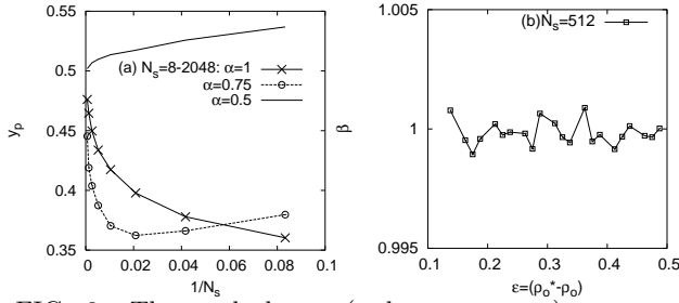
FIG. 6. The parked car (order parameter) exponents (a) y_p = 0.495(5) and (b) \beta = 0.997(3) , at \rho_o = 1/2 and \alpha = 1 of the N - MC phase boundary. For other two curves in (a), taken along the MC - N phase boundary at \alpha \geq 1/2 , the exponent y_p retains the same value, but is subject to large/small corrections to finite-size scaling originating from 2/3 power-law density profile at the beginning of the road (garage exit).
