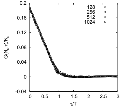
FIG. 10. The parked car correlator G(N_s, \tau) in the C phase; it decays linearly as function of \tau and becomes zero after one time of flight T = N_s/v_g (= \tau_{\text{flight}}) . Since it grows linearly with system size N_s , we plot G/N_s . The data are obtained at \rho_o = 0.75 and \alpha = 0.25 .
