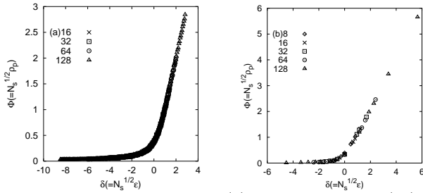
FIG. 7. Scaling function \Phi(\xi) defined in Eq. (17) at the same transition points as in the previous two figures; (a) \rho_o = \alpha = 0.25 ( C - N ) and (b) \rho_o = 1/2 , \alpha = 1 ( MC - N ). The numerical data collapse very well for x_p = y_\epsilon = 1/2 , as suggested in Eq. (17). The scaling function \Phi(\xi) \rightarrow 0 for \xi \ll 0 and \Phi(\xi) \rightarrow \xi for \xi \gg 0 .
