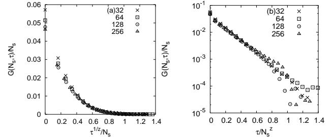
FIG. 15. The parked car correlator G(N_s, \tau) at the MC - N transition; the shape is very similar to that inside the MC phase, see Fig. 9. The data are obtained at \rho_o = 1/2 and \alpha = 1 .
