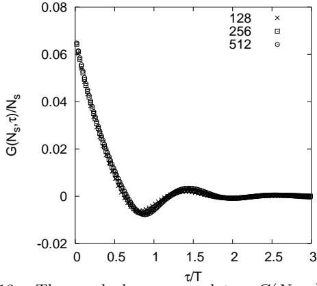
FIG. 12. The parked car correlator G(N_s, \tau) at the C - N transition; it has a strong anticorrelation after one time-of-flight interval, T , even though for small \tau it decays linearly just like in the C phase (and with almost the same group velocity). The data are obtained at \rho_o = \alpha = 0.25 .
