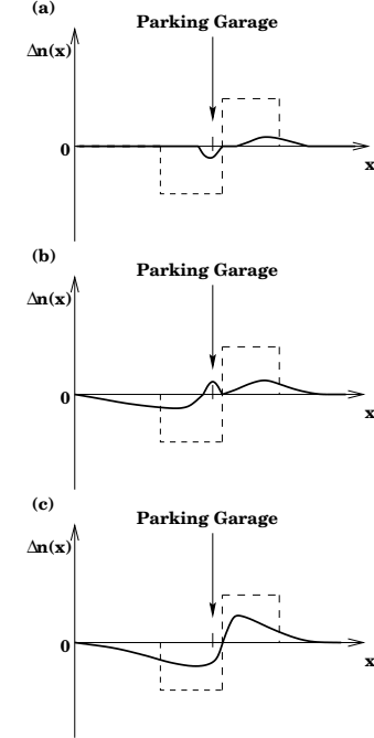
FIG. 14. Schematics of soliton-type local perturbations diffusively spreading from the initial configurations (dashed lines) to one time-of-flight interval later (solid lines); (a) in the C phase, (b) at the C - N transition, and (c) in the N phase.
