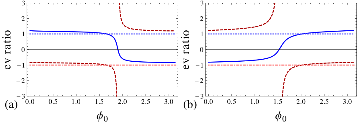
FIG. 6. (Colour online) Ratio between components of each of the two eigenchannel solutions found in the cases with coupled channels. As discussed in the text, if this ratio is close to \pm 1 we have the perfect mixing expected in the SU(4) symmetric limit. (a): \lambda^{(1/2,1/2)} and (b): \bar{u}_2 .
