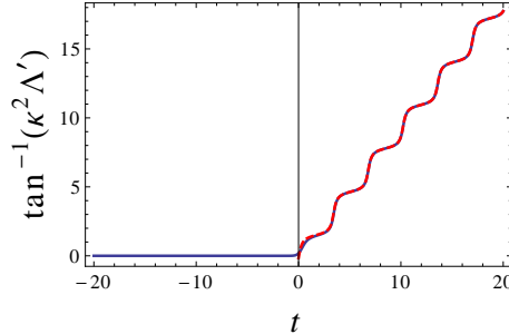
FIG. 1. (Colour online) An example of the full evolution of \Lambda' (solid blue line) compared to the asymptotic evolution (red dashed line). The full evolution was started by integrating downwards from t = 20 , with the same initial condition as chosen for the asymptotic solution.
