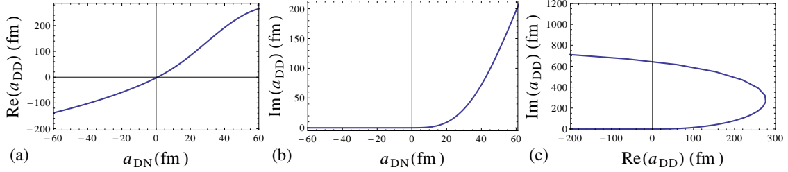
FIG. 4. (Colour online) The relations between the scattering lengths in the SU(4) limit for the channels exhibiting the Efimov effect. All the points on these curves are obtained by choosing different points on the asymptotic limit cycle for \Lambda' as initial values. (a): Real part of dimer-dimer scattering length; (b): Imaginary part of the same scattering length; (c): parametric plot of the real and imaginary parts.
