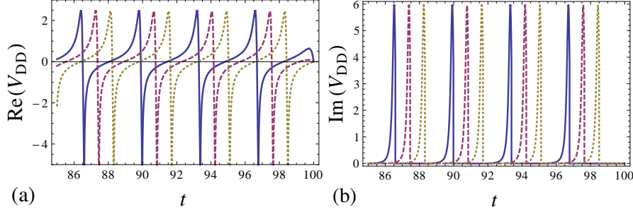
FIG. 2. (Colour online) The evolution of V_{DD} as a function of t in the scaling regime, starting with the initial condition V_{DD} = 0 at t = 100 , for three different choices for the phase of \Lambda' on the asymptotic limit cycle (yellow dotted, red dashed, solid blue). The imaginary part of \Lambda' at the starting point is the same in the three cases shown. (a): Real part, (b): Imaginary part.
