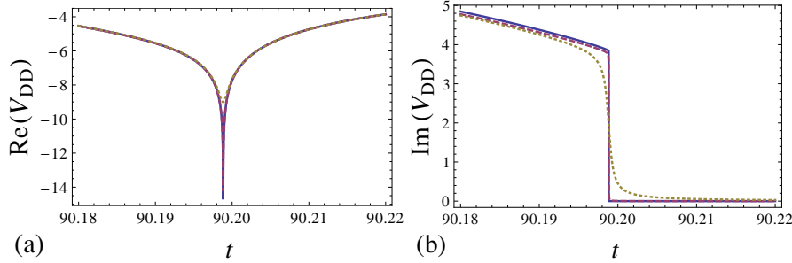
FIG. 3. (Colour online) A single singularity of V_{DD} in the scaling limit, for three decreasing values \delta = 10^{-2}, 10^{-4}, 10^{-6} (yellow dotted, red dashed, solid blue) of the imaginary part in the initial condition on \Lambda' , Eq. (55). (a): Real part, (b): Imaginary part.
