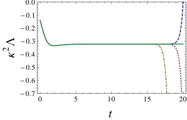
FIG. 8. (Colour online) Four examples of the evolution of \kappa^2\Lambda . These were solved starting the integration at t = \ln \kappa = 20 . The three dashed lines represent the solutions for three random choices of the initial value. The solid (green) line starts using Eq. (A25) as initial condition.
