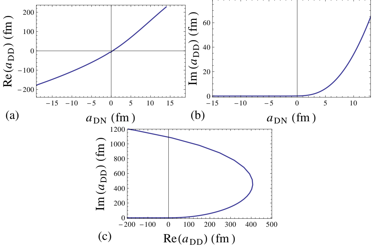
FIG. 7. (Colour online) The relations between the scattering lengths in the Efimov-dominated channels for \alpha = -1/4 . (a): Real part of dimer-dimer scattering length; (b): Imaginary part of the same scattering length; (c): parametric plot of the real and imaginary parts.
