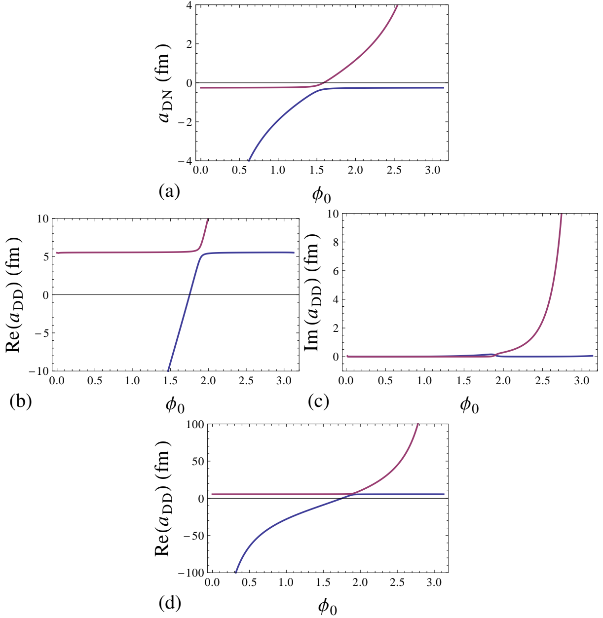
FIG. 5. (Colour online) Evolution of the eigenvalues of the T -matrix (parametrised as scattering lengths) in the two A = 3 ( 1/2, 1/2 ) eigenchannels, and similar for the two A = 4 ( 0, 0 ) eigenchannels, as a function of the parameter \phi_0 specifying the initial condition on the limit cycle. (a): Nucleon-dimer scattering length (which is real), (b): Real part of the dimer-dimer scattering lengths (fine scale), (c) Imaginary part of the dimer-dimer scattering lengths, (d): Real part of the same on a course scale, showing the narrowness of the avoided crossing.
