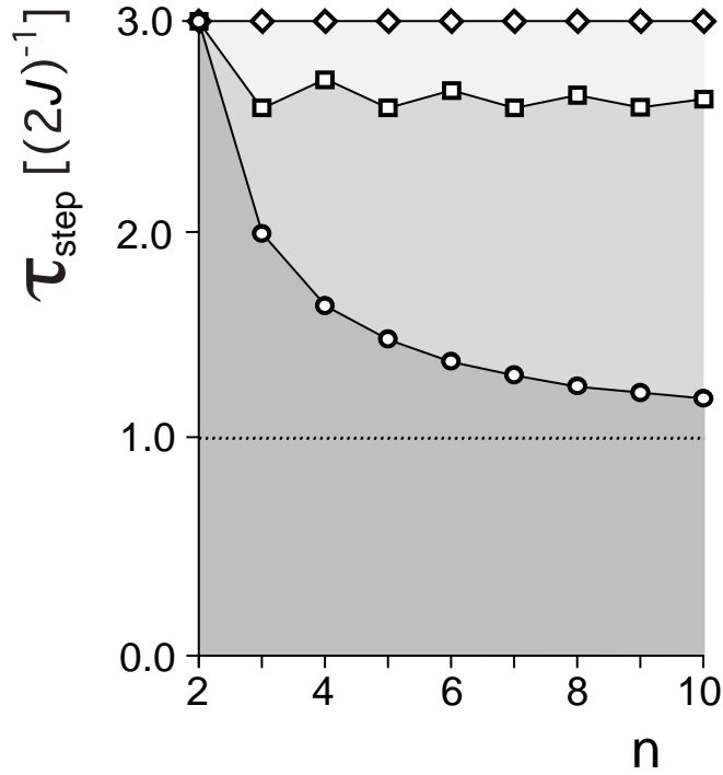
Figure 2: The figure shows a comparison of \tau_{step} = \tau/(n-1) , the average time required to advance by one step in a chain of n coupled spins for pulse sequences which effect full transfer from I_1^- to I_n^- . Diamonds: conventional sequence of selective isotropic mixing steps between neighboring spins [22, 23]. Squares: Sequence of optimal indirect SWAP( k, k+2 ) operations [25] (of duration \frac{3\sqrt{3}}{2J} ) which are followed by a selective isotropic mixing steps between spins (n-1) and n if n is even. Circles: Soliton pulse sequence.
