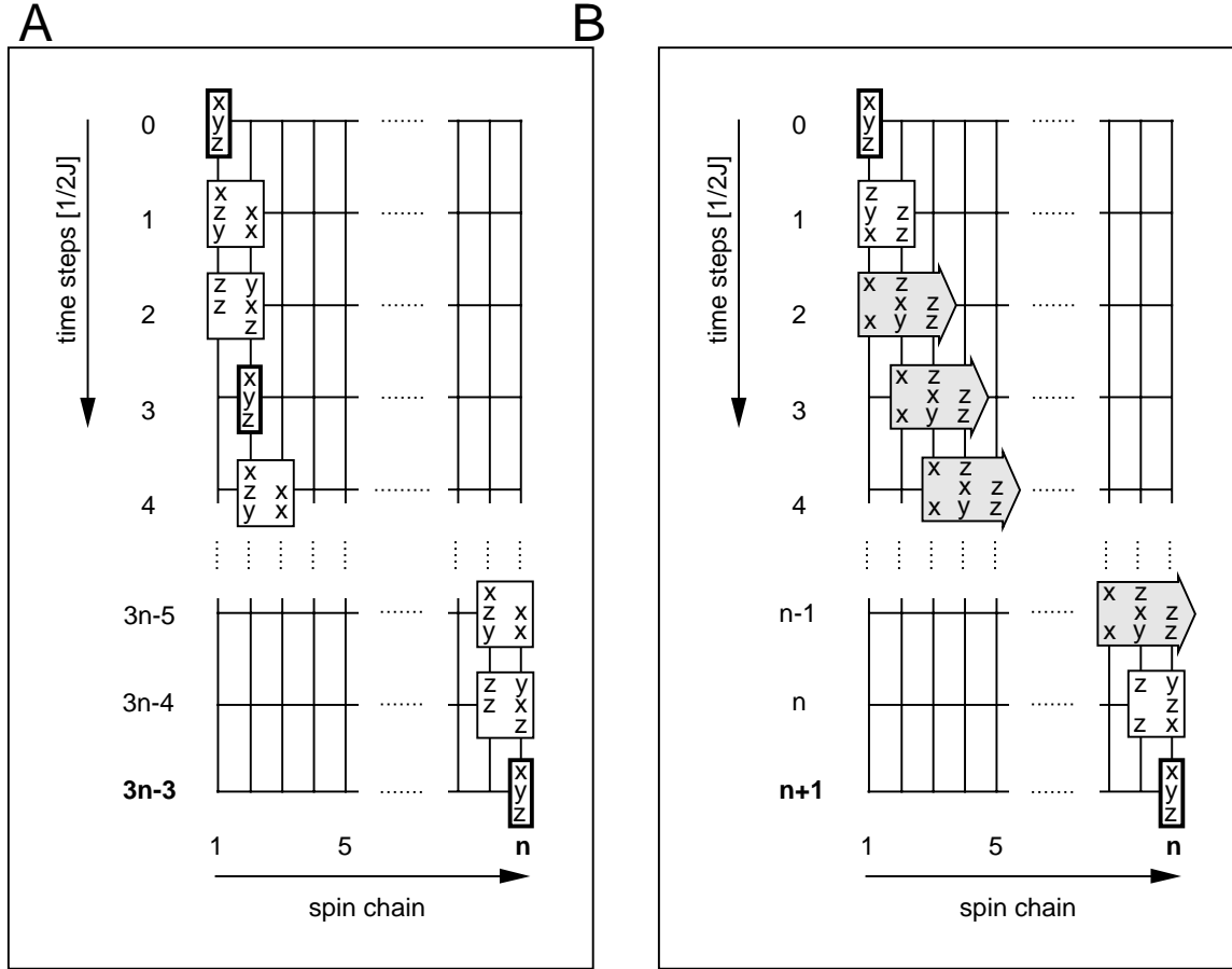
Figure 1: Panel A shows the flow of coherence and polarization in a spin chain under a sequence of selective isotropic mixing periods [11, 22, 23], (sequential swap operations) each of which can be decomposed in three steps of duration \Delta = (2J)^{-1} with effective Hamiltonians 2\pi JI_{(k-1)x}I_{kx} , 2\pi JI_{(k-1)y}I_{ky} , and 2\pi JI_{(k-1)z}I_{kz} , respectively. After the first step the initial operators I_{1x} , I_{1y} , I_{1z} are transferred to I_{1x} , 2I_{1z}I_{2x} , 2I_{1y}I_{2x} respectively. Coherence is transferred in a sequential manner where the state of the spin k is transferred to spin k+1 in \frac{3J}{2} units of time. The total transfer takes \frac{3(n-1)}{2J} units of time. Panel B shows the flow of coherence and polarization under the proposed pulse sequence based on effective soliton operators (indicated by grey arrows). Here, a localized spin wave is created which moves one step in the spin chain in every \frac{1}{2J} seconds. The total transfer time for the proposed pulse sequence is \frac{n+1}{2J} . For clarity, operators such as I_{kx} are indicated by the letter x at position k . Similarly, bilinear (or trilinear) product operators such as \Lambda_{kx} (or \Lambda_{kz} ) are indicated only by the axis labels x , y , or z at the corresponding spin position, omitting prefactors of 2 (or of 4) and possible algebraic signs.
