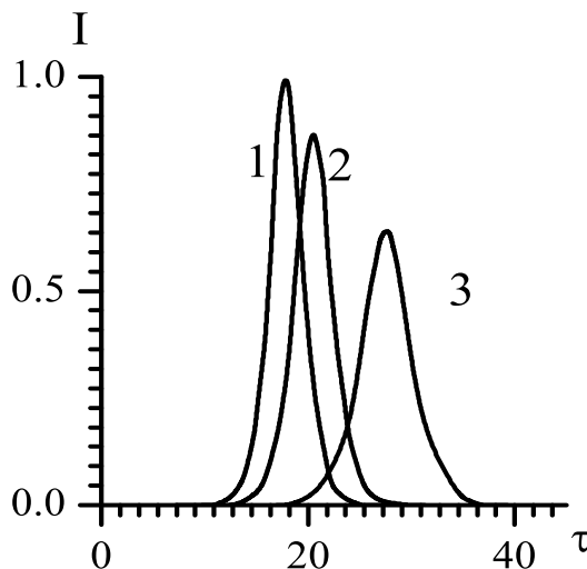
The intensity I of Dicke superradiance (normalized to N\omega_0/4\tau_R^0 ) as a function of \tau = t/\tau_R^{(0)} for three values of the energy W of the excitation laser pulses: 1), W = 0 ; 2), W = 1.25 \times 10^{-3} J ; and 3), W = 2.25 \times 10^{-3} J ( N = 10^{18} ).
