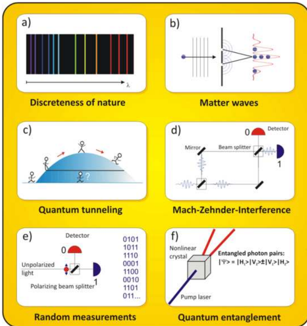
Figure 1: Review of some prominent quantum phenomena: a) Quantum physics emphasizes that our world is built on discrete particles that are bound in finite systems of discontinuous energies. This becomes evident in the finite number of wavelengths \lambda , respectively colors, that an atom emits. (b) The quantum delocalization and wave-particle duality of light and matter can be demonstrated using a double-slit experiment (see text). (c) Quantum wave effects allow tunneling through an energy barrier which would classically be insurmountable. (d) A Mach-Zehnder interferometer allows to split a wave into two widely separated paths. (e) A quantum measurement generates objective randomness. A photon beam, that is divided by a 50/50 beam splitter, will hit either detector randomly, and yield an absolutely random sequence of zeros and ones. (f) Entanglement is the inseparable quantum correlation of two or more particles or degrees of freedom. Here, we sketch the creation of a polarization entangled pair of red photons when a single uv pump photon interacts with a nonlinear crystal (Kwiat et al., 1995). A measurement of both photons shows perfectly anti-correlated polarizations although the result on each side individually appears to be absolutely random.
