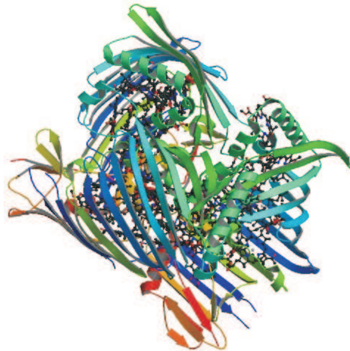
Figure 4: The Fenna-Matthews-Olson (FMO) complex is composed of three protein-pigment structures. Each of them contains seven bacteriochlorophyll-a molecules (Blankenship, 2002). Electronic excitation transfer from the FMO complex to the reaction center is a key process in the light-harvesting of green photosynthetic bacteria. Two dimensional Fourier-Transform spectroscopy (Engel et al., 2007) was able to document long-lived excitonic coherences across neighboring molecules in this structure (picture credits: Tronrud et al., 2009).
