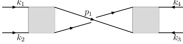
Figure 3: An example of a four-point Feynman graph, planar but with 2 faces broken by external lines
