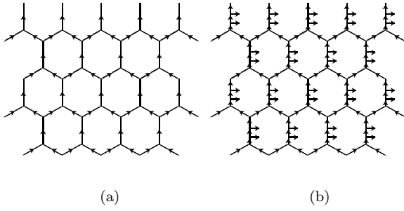
FIG. 3: Extension of the Hilbert space by extra tails.
