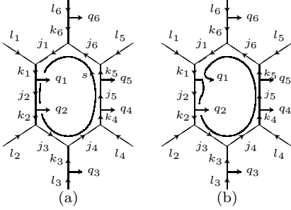
FIG. 12: (a) \tilde{\mathcal{B}}_p^s creates a Wilson loop labeled by s ; (b) the twist \Theta_{vp} of the charge q_1 moves q_1 around the plaquette.
