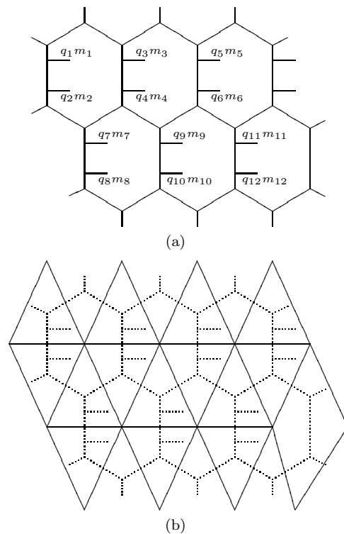
FIG. 17: (a). The Hilbert space for Rep_H model on trivalent graph \Gamma , with each tail labeled by q_v, m_v . (b) The Hilbert space for Vec_H model on the triangulation (solid line) dual to \Gamma , with local Hilbert space \mathbb{C}[H] on each edge.
