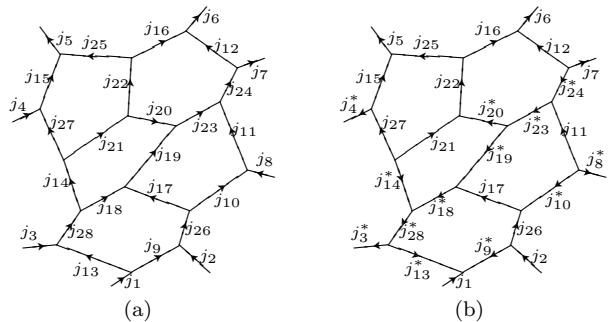
FIG. 1: A configuration of string types on a directed trivalent graph. The configuration (b) is treated the same as (a), with some of the directions of some edges reversed and the corresponding labels j conjugated j^* .
