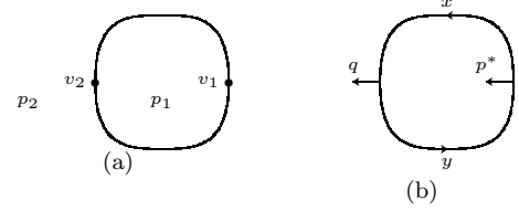
FIG. 13: (a) A circle with two two-valent vertices on the sphere, with two vertices v_1, v_2 and two plaquettes p_1, p_2 . (b) Circle with two tails.
