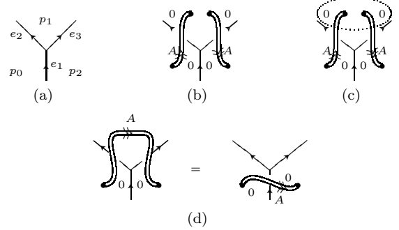
FIG. 15: (a) Three neighboring plaquettes around a trivalent vertex. (b) Create two fluxon pairs across the edge e_2 and e_3 . (c) Annihilate fluxons at p_1 by n_{p_1}^0 . (d) The final fluxon-pair state in (c) is equal to that obtained by directly creating a fluxon pair across edge e_1 . This implies n_{p_1}^0 W_{e_2}^A is path independent, and thus is a hopping operator of fluxon A at p_1 .
