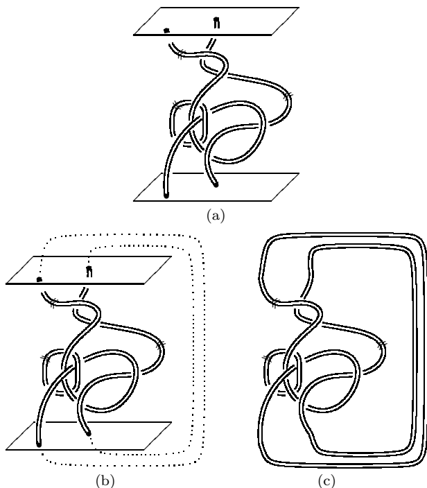
FIG. 18: (a) A tangle representing f_L , which is the creation of a dyon-pair from a ground state. (b) Illustration of gluing dots along S^1 . (c) Closure of underlying topological object is L .
