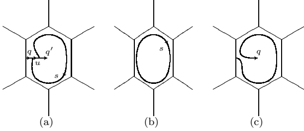
FIG. 5: Graphical interpretation of B_{qq's} and B_p^s . (a) B_{qsq'u} attaches a string and fuses it along the plaquette boundary by \hat{T}_1 and \hat{T}_3 . (b). With q = q' = 0 , B_{qq's} is reduced to B_{0s0s} = \mathcal{B}_p^s . (c) With u = 0 , \Theta performs a rotation of a tail along the plaquette boundary.
