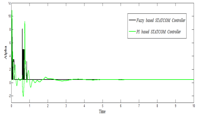
Fig 13. Alpha with time.
