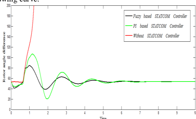
Fig 7. Rotor angle difference with time.
