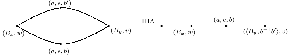
Figure 2: A fold of type IIIA
