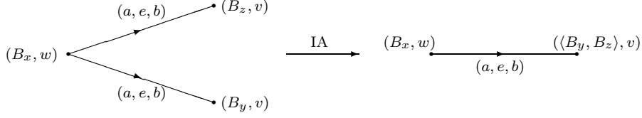
Figure 1: A fold of type IA
